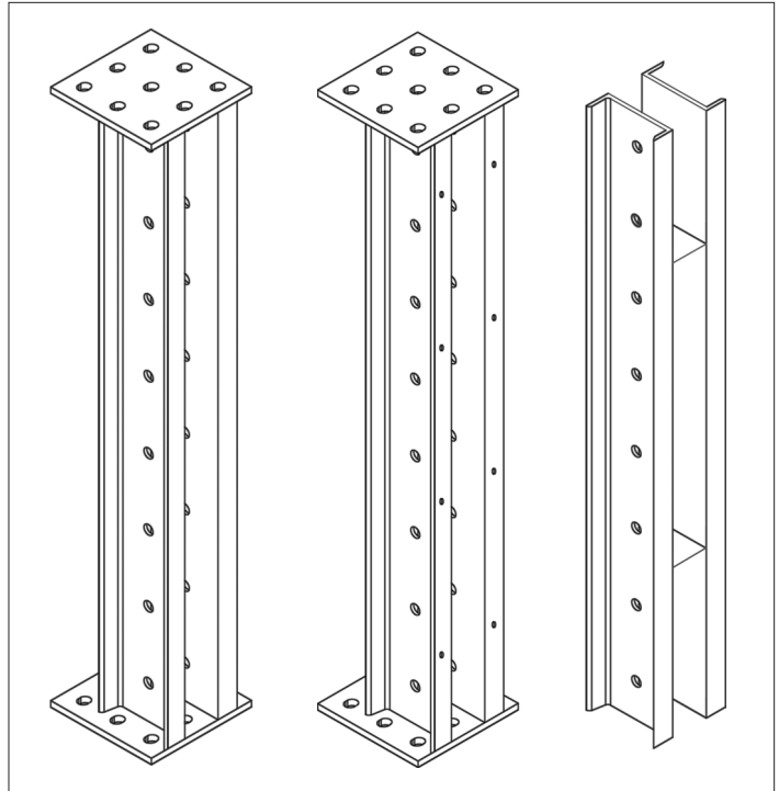
Walers (left to right) - Butt Plate Waler, Pafco-style Waler and Double Channel Waler.
